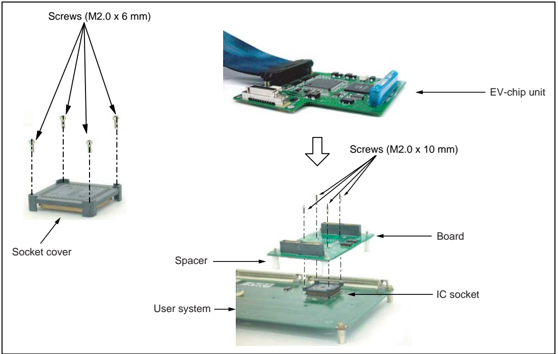
Figure 1 User System Interface Board for the SH7125 PRQP0064GB-A (Former Code: FP-64AV) Package
